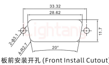
板前安装开孔 (Front Install Cutout)
